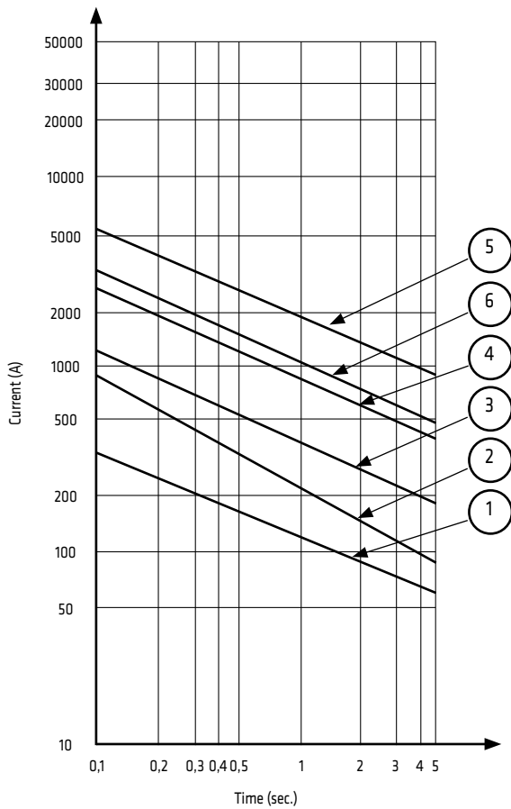
DIAGRAM OF PEAK CURRENTS
