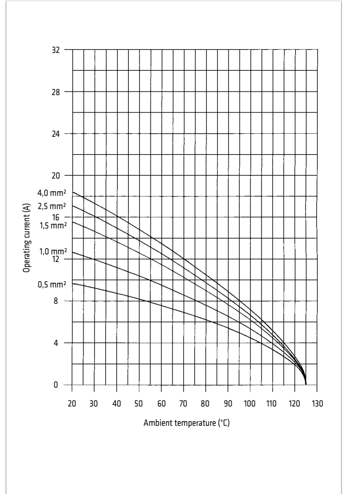
GW-E, GW-EAV RANGE 24/28P + \frac{1}{2}
