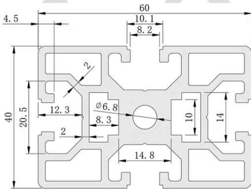
Cross section of bracket
