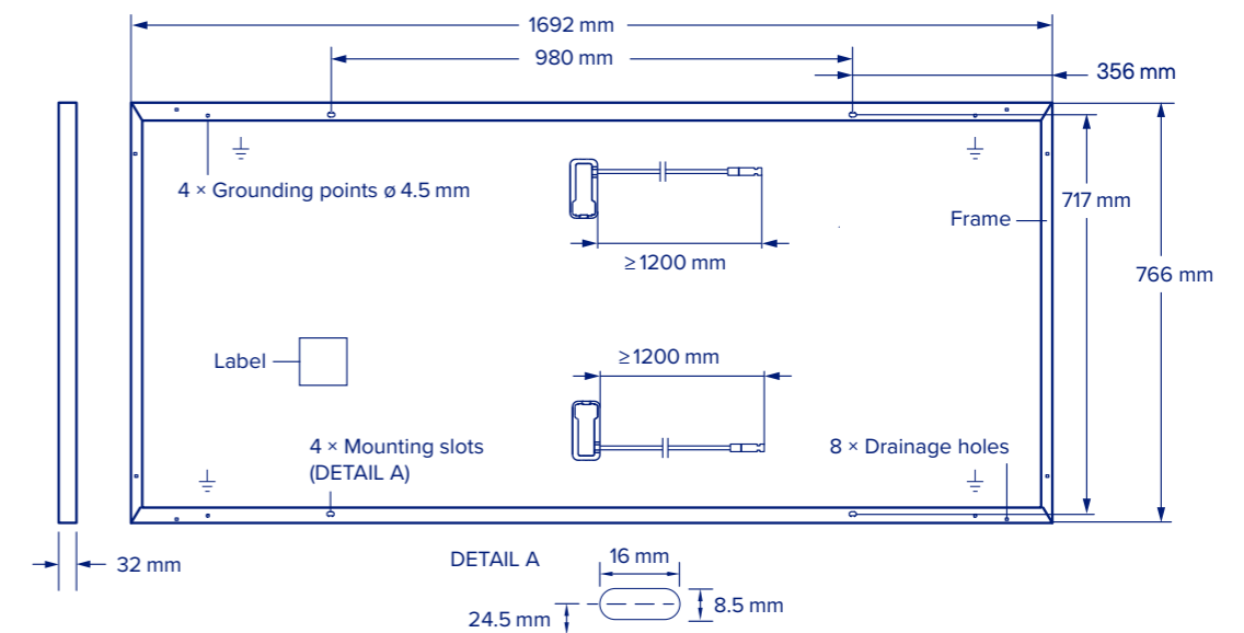
Fig. 1: External dimensions (in mm) and components for Q.PEAK DUO S-G11.
